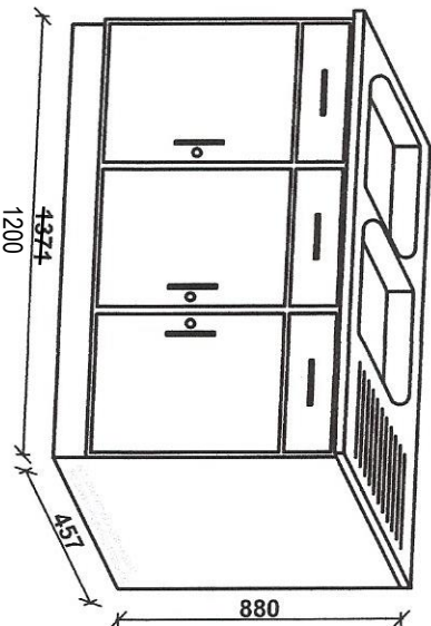
SINK UNIT 1374mm Changed to 1200mm
